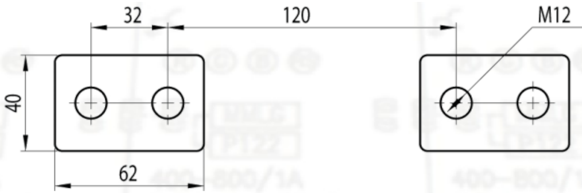
implementation of primary terminals up to 1250 A according to IEC
